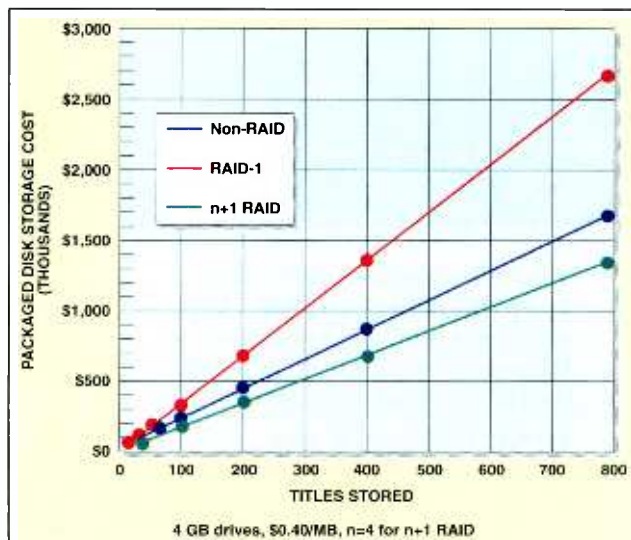
Figure 2. This chart shows the typical storage costs for varying number of compressed (3Mb/s video rate) 2-hour movies. Shown are costs for non-redundant, n+1 RAID and mirroring (RAID-1) configurations.
